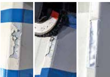
Figure 1 Grind/clean area for bonding.
